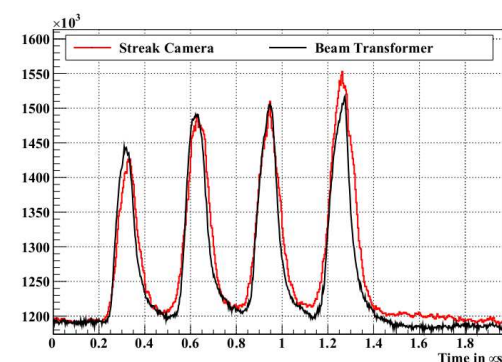
Figure 2: Comparison between the signal recorded with the beam transformer in the extraction beam line and the projection of a single streak picture onto the time axis for a U^{29+} -beam in arbitrary units.
