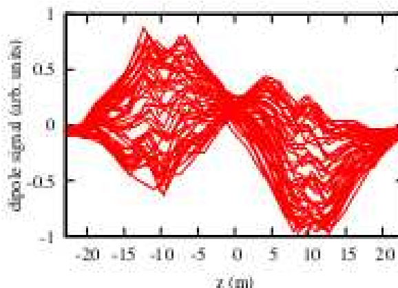
Figure 2: Traces of the transverse bunch signal for 50 consecutive turns. This result proves that the k = 1 remains during the process of bunch decoherence in the case of strong transverse nonlinearity.
