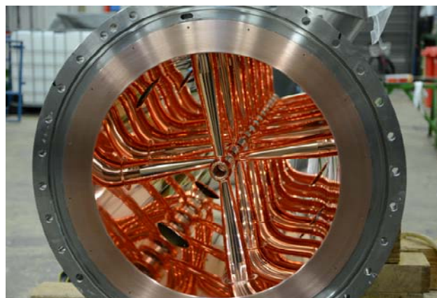
Figure 2: Shiny Copper plated prototype CH-Cavity.
