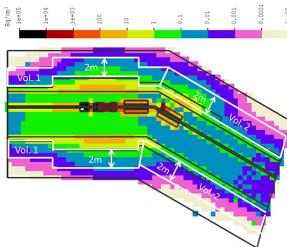
Fig. 2: Level of the activity concentration in units of \text{Bq/cm}^3 calculated for an Uranium beam of 1 GeV/u and a loss rate of 30 % at the ESS of SIS18 beam tunnel.
