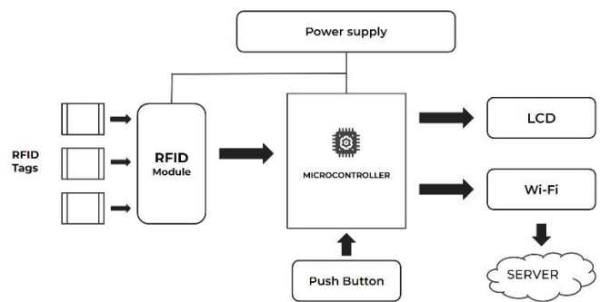
Fig.7. Design of the model proposed
