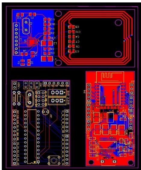
Fig.6. PCB design
