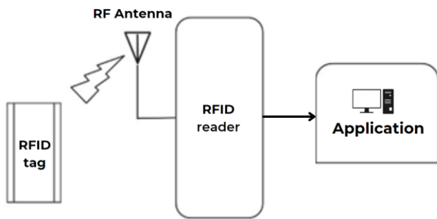
Fig.3. Working of the RFID module
