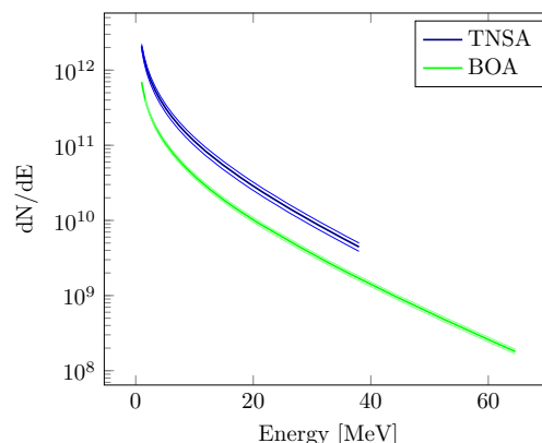
Figure 1: Particle distribution function dN/dE of laser-driven protons obtained from a 700 nm thick plastic target at PHELIX using radiochromic film. The blue and the green lines correspond to protons accelerated via the TNSA and BOA acceleration schemes, respectively.
