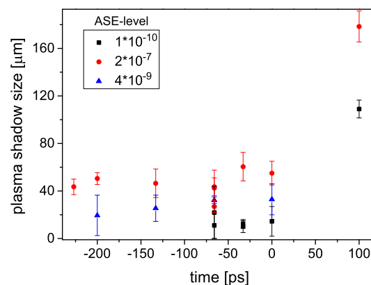
Figure 2: Size of the preplasma shadow for different times and three different ASE-levels
