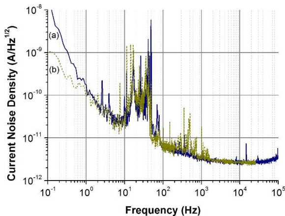
Figure 5: Current noise density of the FAIR-CCC without the matching transformer (a) whereas trace (b) represents current noise density of the FAIR-CCC with matching transformer.
