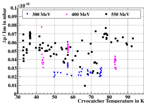
Figure 6: Effective pressure rise as a function of the cryocatcher’s temperature for different Bi-beam energies.
