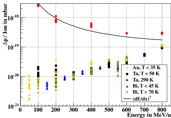
Figure 5: Effective pressure rises as a function of the beam energy for all measurements and different cryocatcher temperatures.
