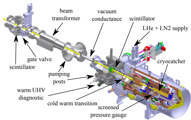
Figure 3: 3D-sctech of the prototype cryocatcher test setup.
