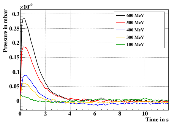
Figure 4: Some exemplarily pressure developments after beam impact onto the cryocatcher for different Bi-beams.
