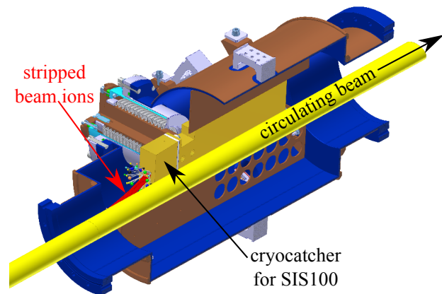
Figure 1: 3D-modell of the cryocatcher prototype with surrounding UHV-chamber (blue) made of stainless steel with an explosively plated copper surface (brown).
