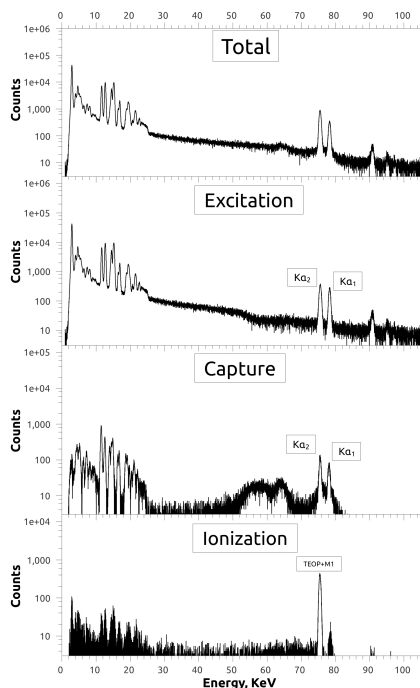
Figure 1: Preliminary x-ray spectra recorded for \text{Bi}^{79+} \rightarrow \text{N}_2 (see text for details).
