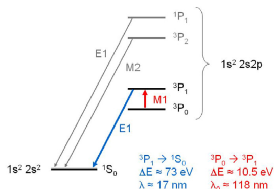
Figure 2: Excerpt of the level-scheme of beryllium-like krypton.
