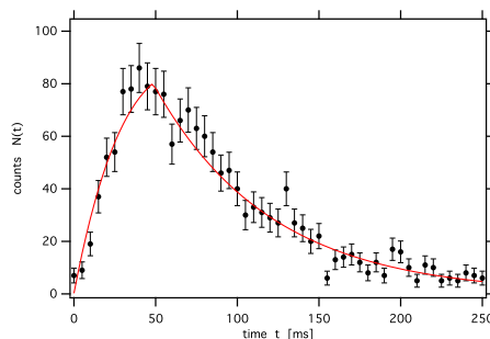
Figure 2: Decay spectra of the \alpha -emitter 221 Ac (half life 52 ms) as a function of the time after injection of each ion bunch in the CSC.
