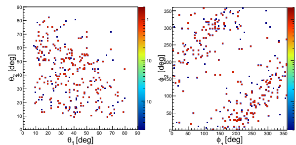
Figure 3: Angular correlations of protons from the CH 2 target and neutrons from the projectile 23 O. Left: polar-angle correlations; right: azimuthal-angle correlations.
