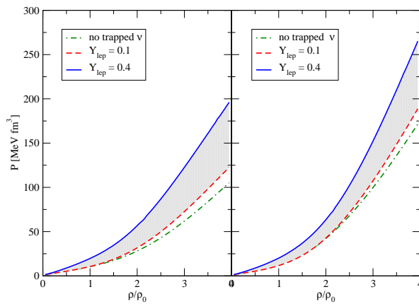
Figure 1: Equation of state in the DD-ME2 parametrization in presence of hyperons. Left panel: we fix the coupling constant g_{\Lambda\Lambda\sigma} = 0.58g_{NN\sigma} from NSC89 potential and we vary the couplings for the \Sigma and \Xi hyperons. The dashed area shows the variation of the EoS with the variation of the coupling constants of the remaining hyperons with the scalar meson. Right panel: the same as the left panel, but for a fixed coupling constant g_{\Sigma\Sigma\sigma} = 0.448g_{NN\sigma} .
