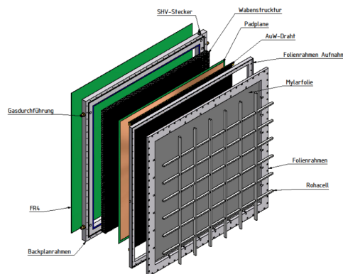
Figure 1: Technical drawing of a full-size TRD-prototype without drift region.
