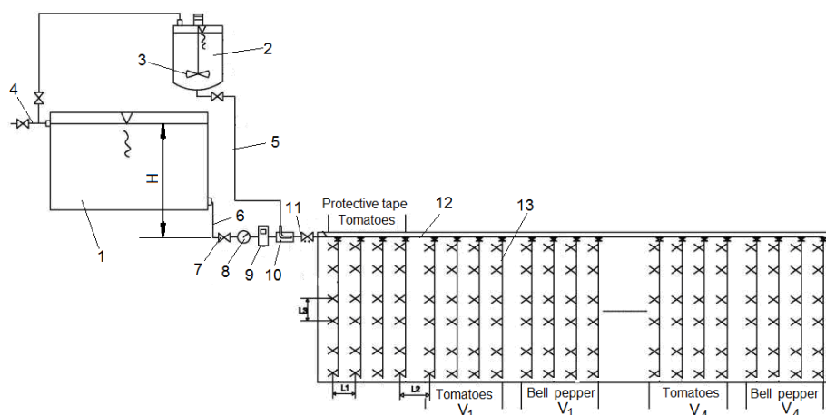
Fig 1 - Experimental setup
