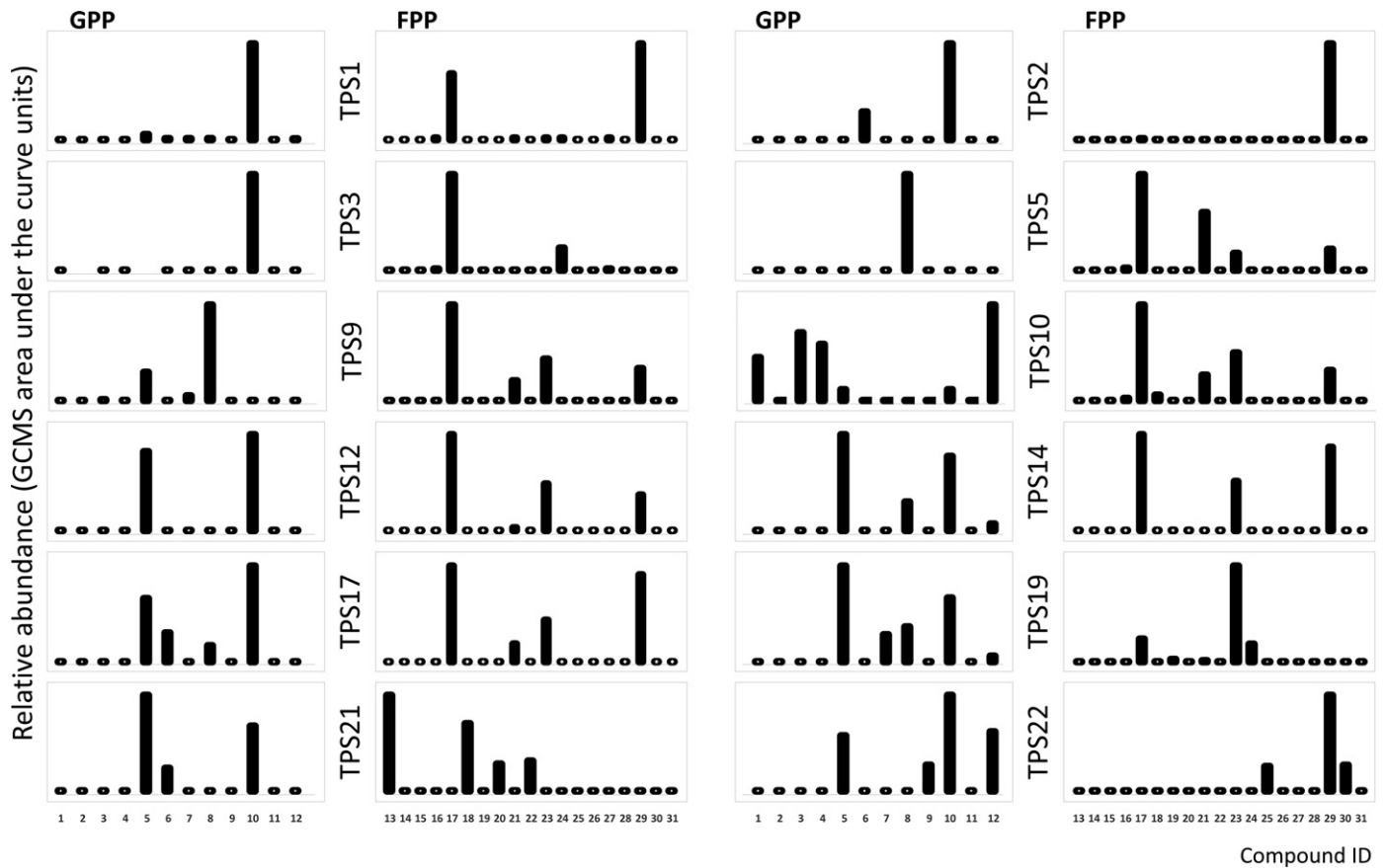
Fig. 4 Products formed in vitro by CstPS2, CstPS3, CstPS5, CstPS9, CstPS10, CstPS19, CstPS21 and CstPS22 upon incubation with geranyl diphosphate (GPP) or farnesyl diphosphate (FPP). Bars indicate the relative abundance of reaction products. Compounds are indicated in numbers as follows: 1, \alpha -pinene; 2, \alpha -phellandrene; 3, sabinene; 4, \beta -pinene; 5, myrcene; 6, limonene; 7, (Z)- \beta -ocimene; 8, (E)- \beta -ocimene; 9, terpinolene; 10, linalool; 11, unknown monoterpene (calculated retention index 1169); 12, \alpha -terpineol; 13, (E)-caryophyllene; 14, (Z)- \beta -farnesene; 15, \alpha -bergamotene; 16, geranyl acetone; 17, (E)- \beta -farnesene; 18, \alpha -humulene; 19, unknown sesquiterpene (calculated retention index 1485); 20, unknown sesquiterpene (calculated retention index 1490); 21, (Z,E)- \alpha -farnesene; 22, unknown sesquiterpene (calculated retention index 1500); 23, (E,E)- \alpha -farnesene; 24, \beta -bisabolene; 25, cadinene; 26, (Z)-nerolidol; 27, (Z)- \alpha -bisabolene; 28, unknown sesquiterpene (calculated retention index 1556); 29, (E)-nerolidol; 30, cadinol; 31, epi- \alpha -bisabolol. Supporting Information Fig. S4 shows the GC-MS chromatograms for CstPS2, CstPS9 and CstPS19 incubated with different substrates. Product profiles of other enzymes that were characterized can be found in Table S6.
