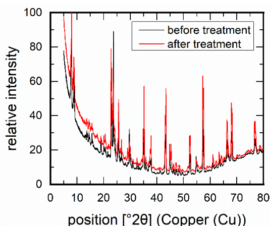
Figure 4. XRD measurements on an MFI membrane before and after amine treatment (2.97 g/L piperazine and 5.15 g/L diethanolamine for 7 days).
