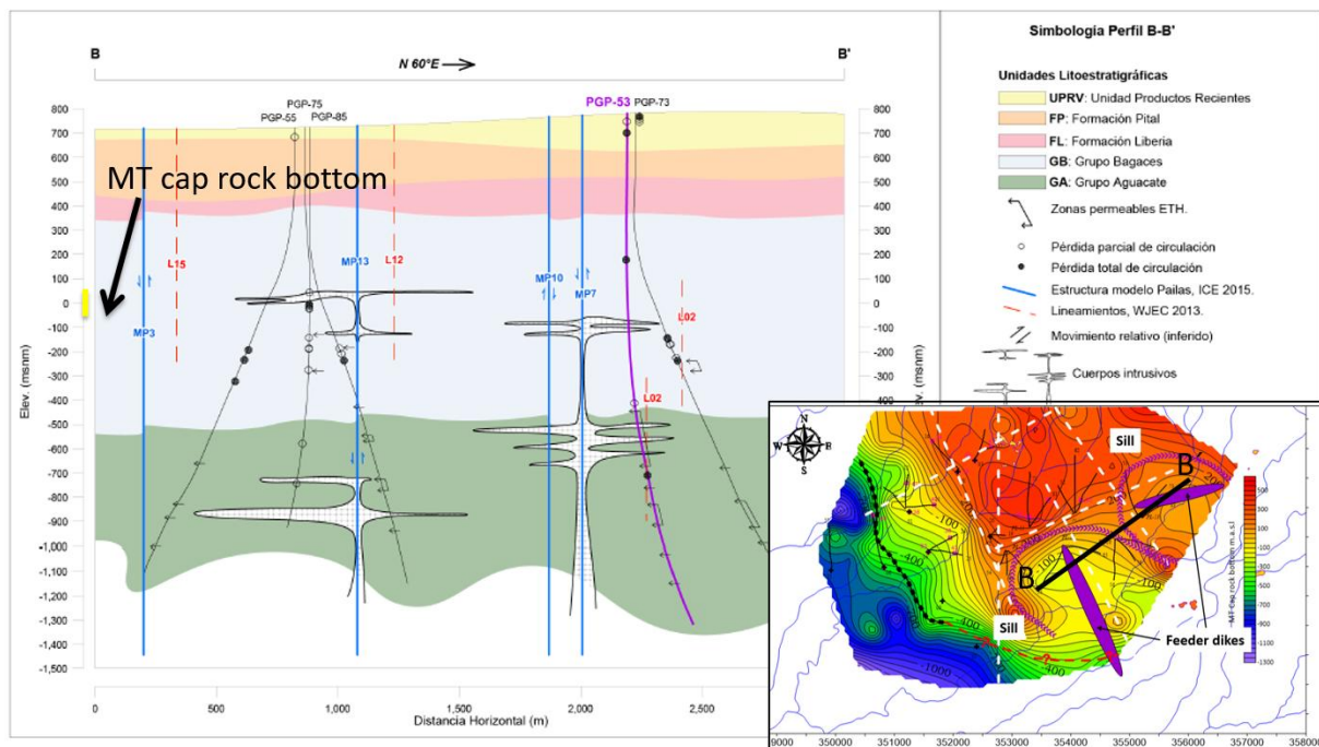
Figure 21. Lithostratigraphic profile B-B' between the wells PGP-55 and PGP-73. The elevation of the MT BOC in the PGP-75 is marked in the section with a small yellow line, corresponding precisely to the
