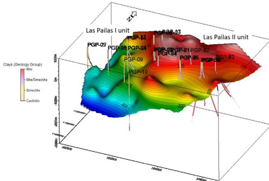
Figure 6. 3D model showing Las Pailas Geothermal Field with geothermal production/injection wells. MT BOC in m.a.s.l shows good agreement with the lower temperature alteration mineralogy (<180°C) represented by the smectite (light yellow) to higher temperatures shown by the appearance of the illite/smectite transition zone (light purple) determined by the ICE Geology group (Costa Rica). Beneath the MT BOC the presence of the high-temperature and -permeability illite (pink) related to highly productive zones can be seen.
