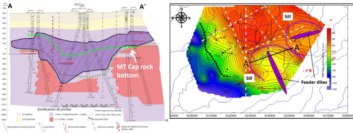
Figure 20. Left picture: Clay zones correlation profile and permeable zones in profile A-A'. A clear chlorite-smectite zone depicted in purple is visible in the profile. The green dot line reveals the contact of the MT BOC according to the section. Right picture: Location of the profile can be seen in the right image. Modified after Gálvez & Ramírez [6].
