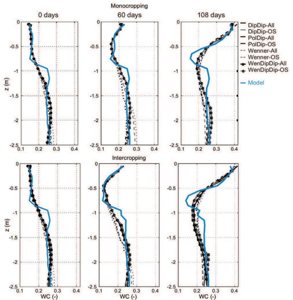
Fig. 7. One-dimensional water content profiles for the mono- and intercropping case at t = 0, 60, and 108 d for a profile of 2-m width and 3-m depth in the middle of the simulated domain. The simulated values are represented by the thick, blue line. DipDip = dipole-dipole, PolDip = pole-dipole, WenDipDip = combination of Wenner & Dipole-dipole. Electrode arrays using only surface electrodes are marked by surface electrodes (OS).
