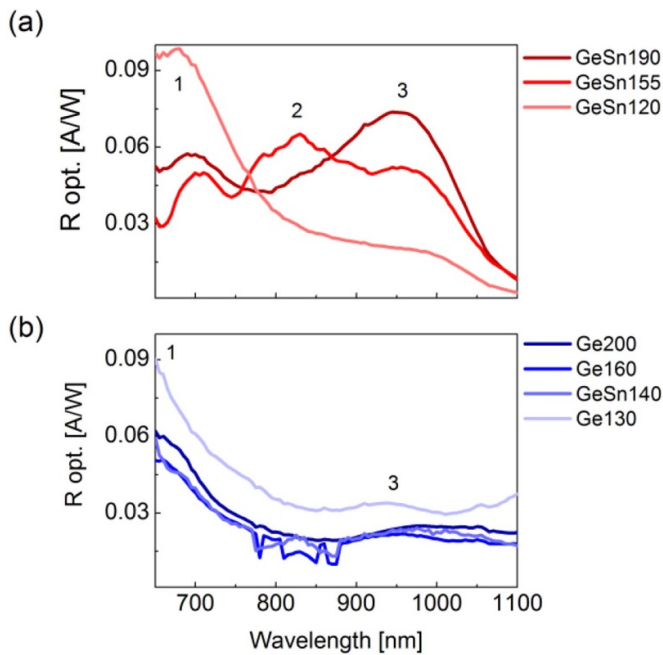
Figure 6. Responsivity spectra R_{opt.} of Ge and GeSn nano-islands on (a) p^- -Si substrate (red graphs) and (b) n^{++} -Si substrate (blue graphs) at position A depending on the wavelength. The increasing island size is indicated as darkening of the color. The different peaks are labeled with numbers from 1 to 3.
