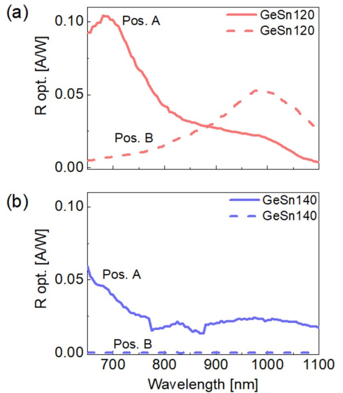
Figure 7. Wavelength-dependent responsivity spectra R_{opt.} of (a) GeSn120 on a p^- -Si substrate (red) and (b) GeSn140 on a n^{++} -Si substrate (blue). Position A (solid graph) corresponds to a region with Al, while at position B (dashed graph) no Al top layer is present.
