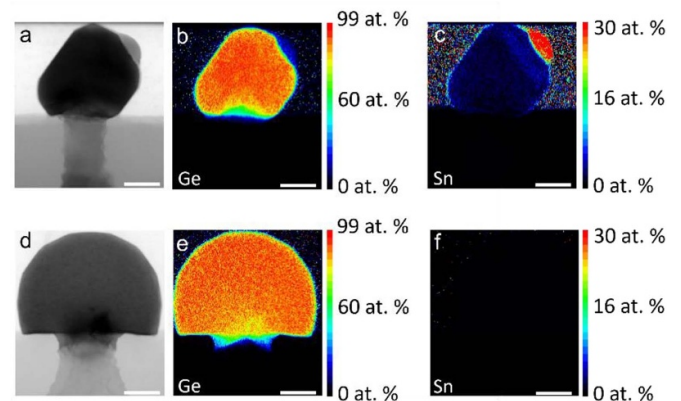
Figure 2. (a) STEM BF image, EDX map of (b) Ge and (c) Sn distribution of GeSn140. The average Sn content within the nano-island is 1.4 \pm 0.5 at.%. (d) STEM BF image, EDX map of (e) Ge and (f) Sn distribution of Ge160. No Sn contamination can be detected in the Ge nano-island. The scale bar of all images is 40 nm.
