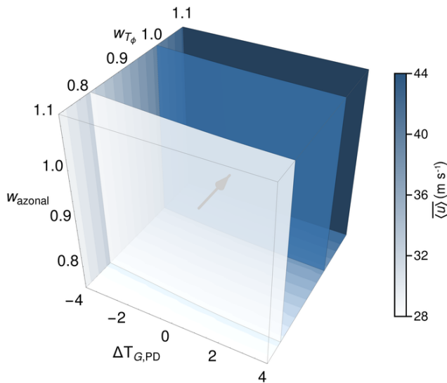
Figure 6. Jet stream strength defined by the maximum of the zonal-mean zonal wind velocity ( \overline{\langle u \rangle} ) between 10^\circ and 80^\circ N at a height of 9000 m (corresponds to 300 mbar) in relation to w_{T_\phi} and w_{azonal} and \Delta T_{G,PD} in boreal winter.
