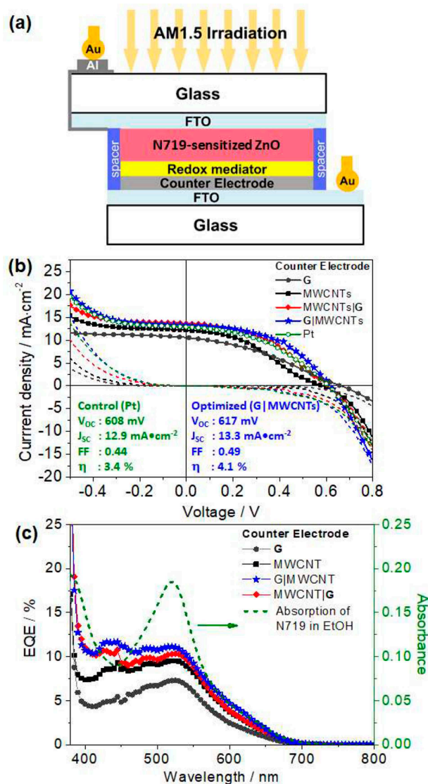
Figure 6. (a) Sandwich structure of ZnO-based DSSC using different counter electrodes, (b) J-V of ZnO-based DSSCs using different counter electrodes measured under 100 mW cm -2 AM1.5 irradiation (solid line) and in the dark (dashed line). (c) EQE curves of ZnO-based DSSCs using different counter electrodes. The counter electrodes used in the DSSC were annealed under N 2 atmosphere.
