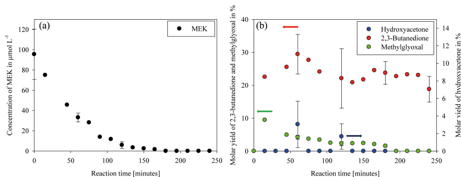
Figure 1. (a) Consumption of MEK during the oxidation with OH radicals and (b) time-resolved formation of the products methylglyoxal, 2,3-butanedione, and hydroxyacetone.
