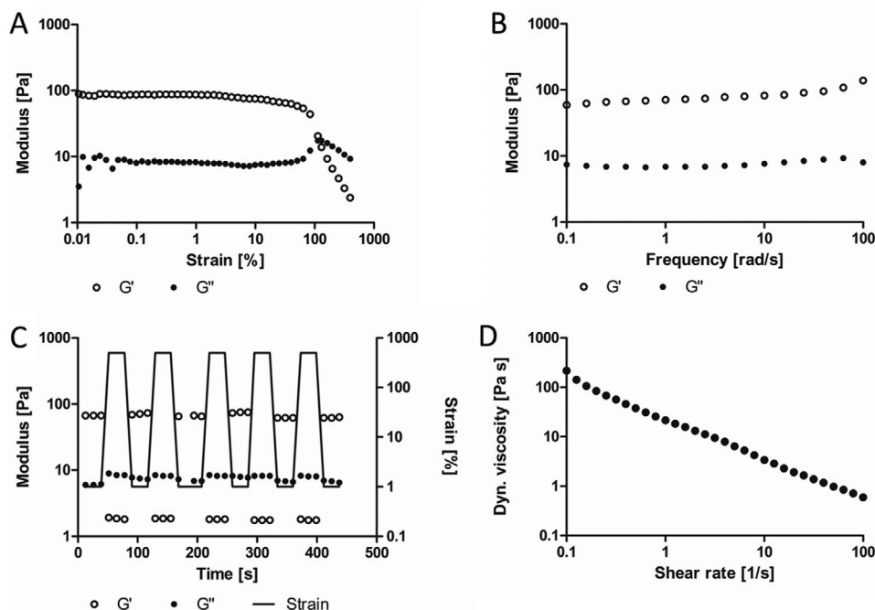
Figure 1. Rheological data of 0.4 mL of 0.6% (w/v) cellulose nanofibril (CNF) hydrogel at 20°C and a plate gap of 0.5 mm. A) Dynamic oscillatory amplitude sweep measurement at 1 \text{ rad s}^{-1} . B) Frequency sweep measurements at 0.5% oscillating strain. C) Altering strain measurement between 1% and 500% in periods of 30 s. D) Dynamic viscosity measurement with 5 s equilibrium time and 30 s averaging time.
