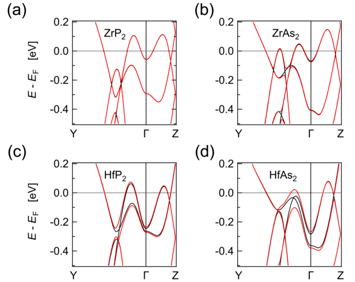
FIG. 5. Gap opening along the nodal loop through increased spin-orbit coupling (SOC). Band structures along Y-\Gamma-Z for (a) \text{ZrP}_2 , (b) \text{ZrAs}_2 , (c) \text{HfP}_2 , and (d) \text{HfAs}_2 . Black lines: without SOC, red lines: with SOC. Experimentally determined crystal structures were used for calculations on \text{ZrP}_2 [40] and \text{ZrAs}_2 [51]. For \text{HfP}_2 and \text{HfAs}_2 , the crystal structures of \text{ZrP}_2 and \text{ZrAs}_2 were used, respectively.
