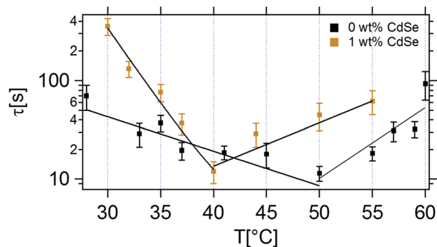
Fig. 5 Time constants of the electric field-induced reorientation at 1 kV mm -1 for a sample of poly(styrene)-block-poly(isoprene) (33.2 wt%) in toluene without nanoparticles (black squares) and with 1 wt% of CdSe quantum dots (orange squares) as a function of temperature.
