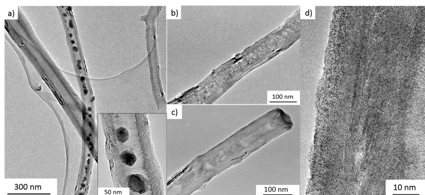
Figure 8. TEM images of (a) uncycled, (b) galvanostatically lithiated, and (c) delithiated \text{Mn}_3\text{O}_4\text{@CNT} . (d) High-resolution TEM image of a CNT shell of delithiated material after 13 cycles. Taken from [45].
