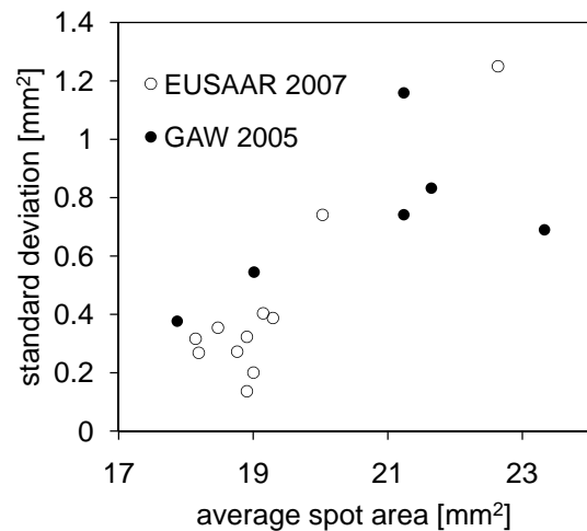
Fig. 5. Standard deviation of PSAP spot area versus average spot area. Each point is for one PSAP. The nominal spot area given by the manufacturer is 17.85 \text{ mm}^2 .
