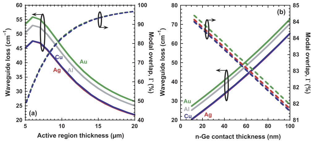
Fig. 3. (a) The waveguide losses and modal overlaps at 300 K for surface plasmon waveguides on a 100\ \mu\text{m} wide ridge with 50\ \text{nm} n-Ge top and bottom contact layers for different \text{Si}_{0.1}\text{Ge}_{0.9} active region thicknesses for four different metals. (b) The waveguide losses and modal overlap for surface plasmon waveguides on a 100\ \mu\text{m} wide ridge with a 10\ \mu\text{m} thick \text{Si}_{0.1}\text{Ge}_{0.9} active region as the n-Ge top and bottom contact regions are varied in thickness.
