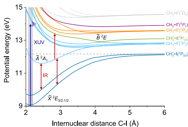
Figure 2. Ab initio potential energy curves (PECs) for the methyl iodide cation at the XMS-CASPT2 level of theory including SOC at PM-CASSCF and relaxing the methyl moiety in the ground state of the cation. The energy origin is taken at the vibrationless electronic ground state of neutral \text{CH}_3\text{I} . The blue vertical arrow indicates one-photon absorption of the 9th harmonic of the fundamental 800 nm (13.95 eV, 88.89 nm). The up and down red arrows show pump and dump processes associated with the interaction with the IR pulse (see the text for more details). The horizontal dashed line shows the first dissociation threshold of the \text{CH}_3\text{I}^+ cation. Notice the overlap between high vibrational states of the \tilde{X}^2E_{3/2,1/2} ground state and low vibrational states of the excited \tilde{A}^2A_1 state below this horizontal dashed line. The grey shaded area represents the Franck–Condon region of the neutral molecule. The Gaussian curve represents the energy width of the 9th harmonic (300 meV full-width-half-maximum).
