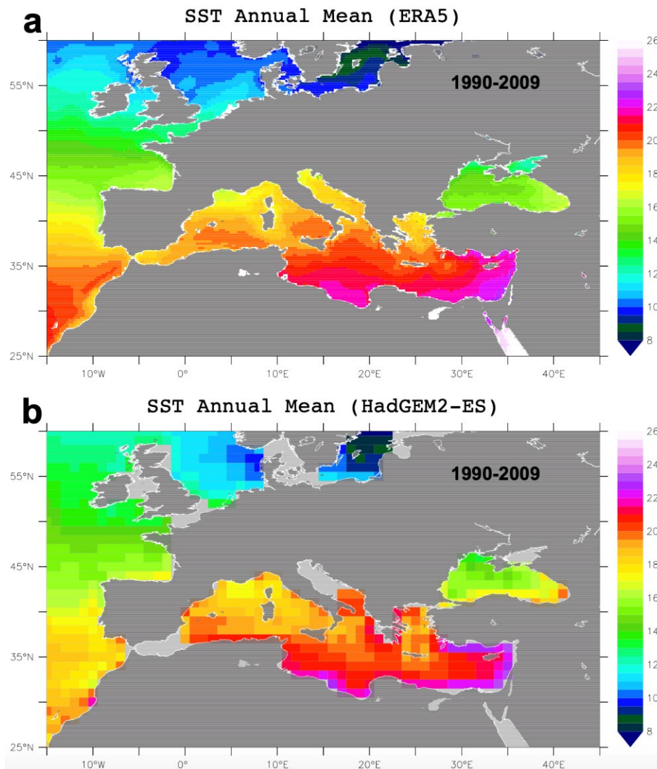
Figure 8. Annual average sea surface temperature for (a) ERA5 and (b) RegCM input for 1990–2009.
