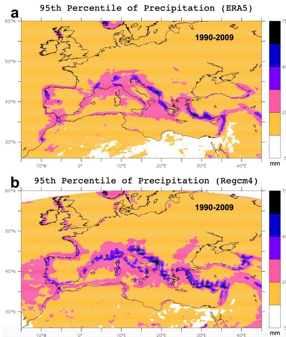
Figure 2. 95th percentile of precipitation for (a) ERA5 and (b) RegCM4 for 1990–2009.
