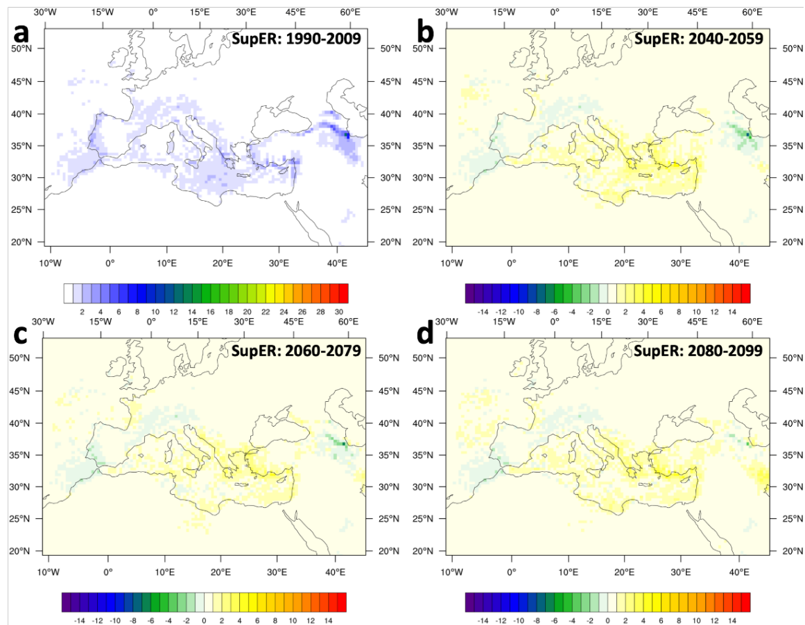
Figure 9. (a) Annual average number of days with CAPE \geq 100 J/kg AND 0–6 km SHEAR \geq 20 m/s AND convective precipitation rate > 0 mm/h (SupER) for 1990–2009, (b) changes in average number of days with SupER for 2040–2059, (c) changes in average number of days with SupER for 2060–2079, (d) changes in average number of days with SupER for 2080–2099.
