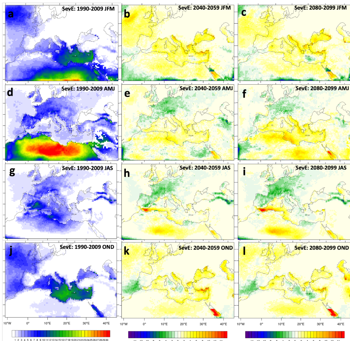
Figure 11. (a) Annual average number of days with CAPE \geq 100 J/kg AND 0-6 km SHEAR \geq 15 m/s (SevE) for January, February, and March (JFM) of 1990–2009, (b) changes in average number of days with SevE for JFM 2040–2059, (c) changes in average number of days with SevE for JFM 2080–2099, (d) annual average number of days with SevE for April, May, and June (AMJ) of 1990–2009, (e) changes in average number of days with SevE for AMJ 2040–2059, (f) changes in average number of days with SevE for AMJ 2080–2099, (g) annual average number of days with SevE for July, August, and September (JAS) of 1990–2009, (h) changes in average number of days with SevE for JAS 2040–2059, (i) changes in average number of days with SevE for JAS 2080–2099, (j) annual average number of days with SevE for October, November, and December (OND) of 1990–2009, (k) changes in average number of days with SevE for OND 2040–2059, (l) changes in average number of days with SevE for OND 2080–2099.
