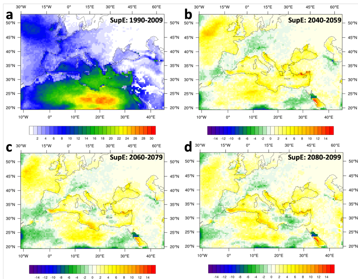
Figure 5. (a) Annual average number of days with CAPE \geq 100 J/kg AND 0\text{--}6 km SHEAR \geq 20 m/s (SupE) for 1990–2009, (b) changes in average number of days with SupE for 2040–2059, (c) changes in average number of days with SupE for 2060–2079, (d) changes in average number of days with SupE for 2080–2099.
