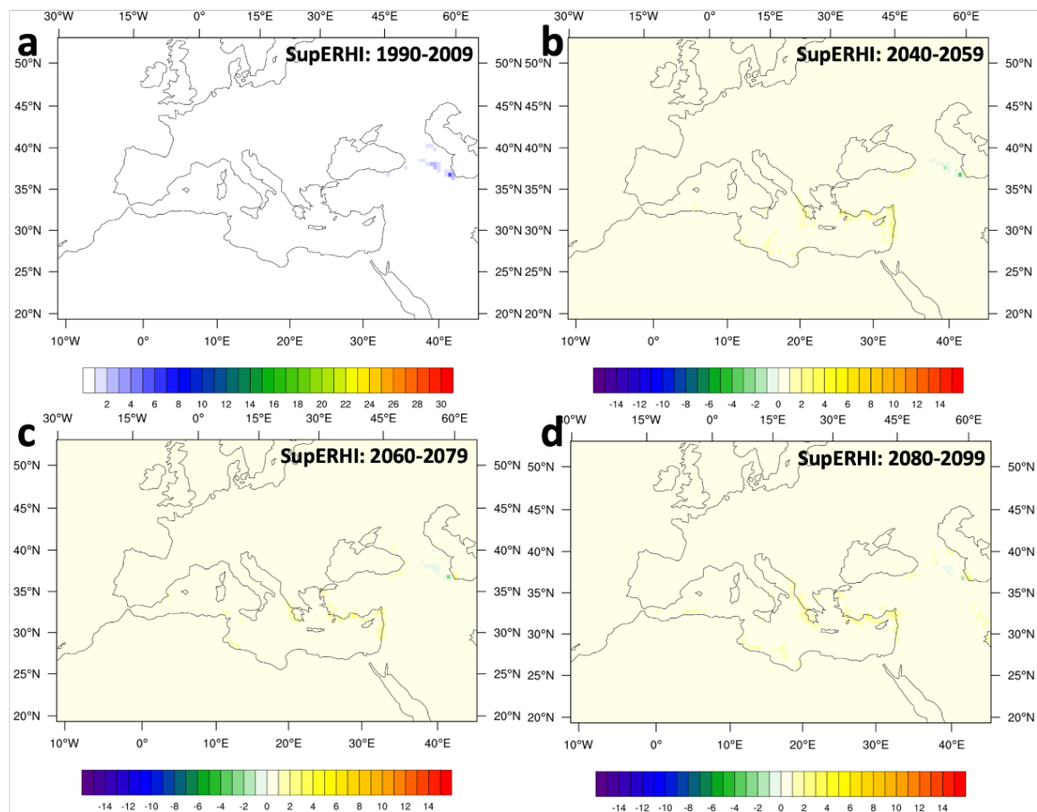
Figure 10. (a) Annual average number of days with CAPE \geq 500 J/kg AND 0–6 km SHEAR \geq 20 m/s AND convective precipitation rate > 0 mm/h (SuperERHI) for 1990–2009, (b) changes in average number of days with SuperERHI for 2040–2059, (c) changes in average number of days with SuperERHI for 2060–2079, (d) changes in average number of days with SuperERHI for 2080–2099.
