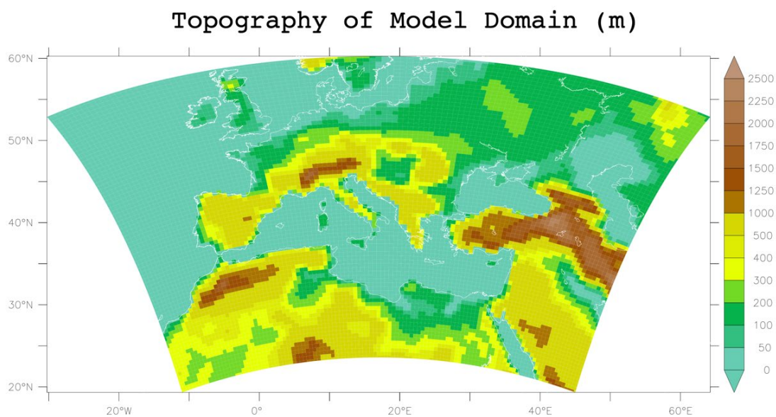
Figure 1. Topography of the domain used in numerical simulations.
