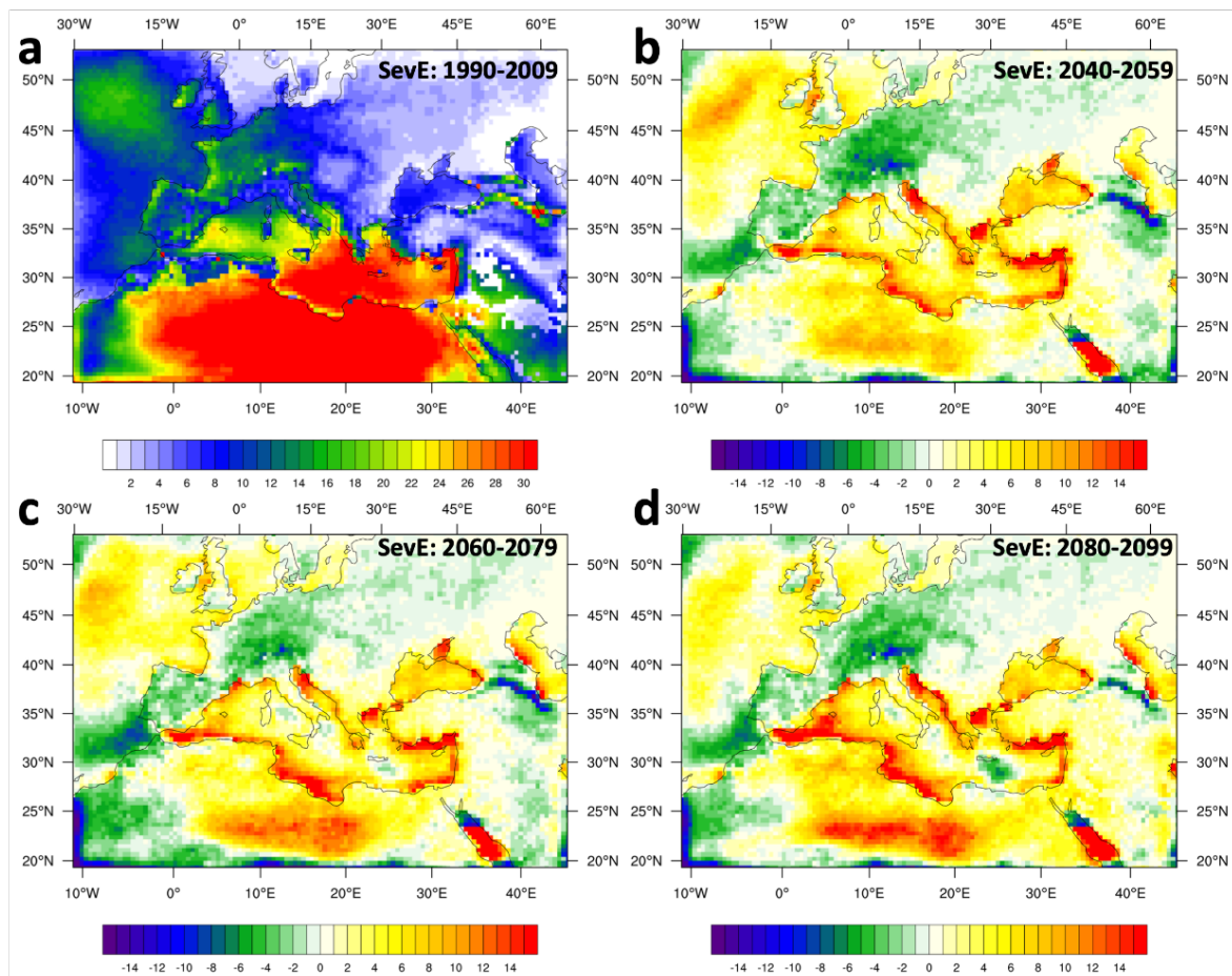
Figure 4. (a) Annual average number of days with CAPE \geq 100 \text{ J/kg} AND 0\text{--}6 \text{ km SHEAR} \geq 15 \text{ m/s} (SevE) for 1990–2009, (b) changes in average number of days with SevE for 2040–2059, (c) changes in average number of days with SevE for 2060–2079, (d) changes in average number of days with SevE for 2080–2099.
