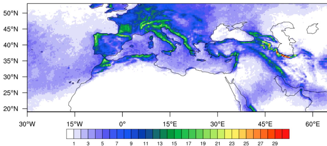
Figure 7. Annual average number of SevER cases calculated with ERA5 data for 1990–2009.
