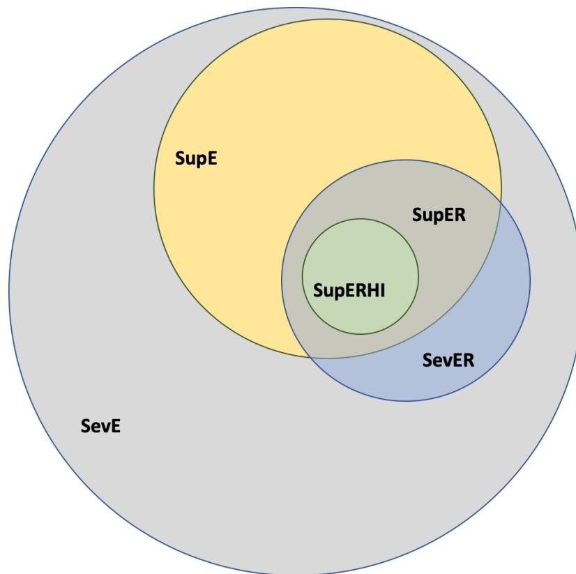
Figure 3. The proxies used in the study (definitions given in Table 1). Areas do not necessarily represent the number of cases.
