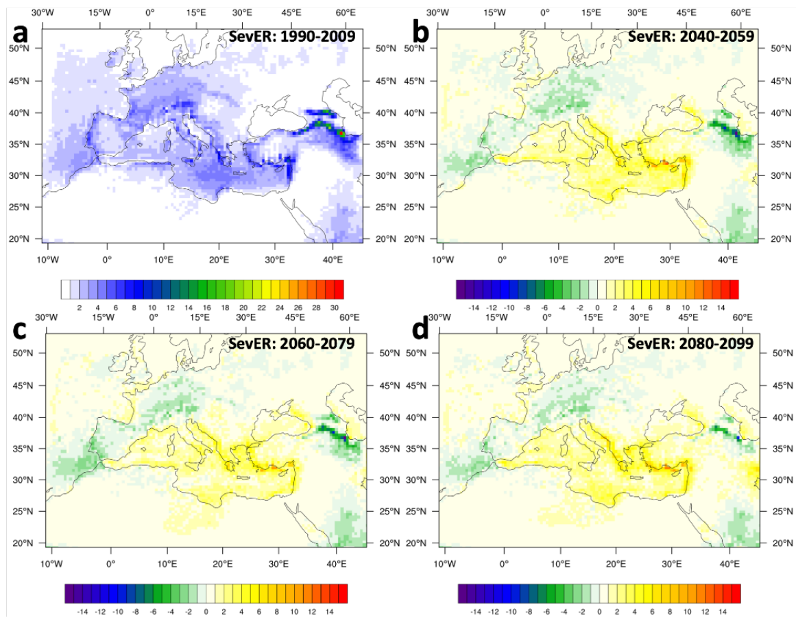
Figure 6. (a) Annual average number of days with CAPE \geq 100 J/kg AND 0–6 km SHEAR \geq 15 m/s AND convective precipitation rate > 0 mm/h (SevER) for 1990–2009, (b) changes in average number of days with SevER for 2040–2059, (c) changes in average number of days with SevER for 2060–2079, (d) changes in average number of days with SevER for 2080–2099.
