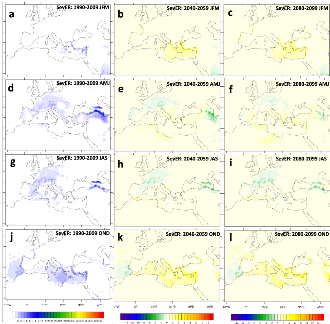
Figure 12. (a) Annual average number of days with CAPE \geq 100 J/kg AND 0–6 km SHEAR \geq 15 m/s AND convective precipitation rate > 0 mm/h (SevER) for January, February, and March (JFM) of 1990–2009, (b) changes in average number of days with SevER for JFM 2040–2059, (c) changes in average number of days with SevER for JFM 2080–2099, (d) annual average number of days with SevER for April, May, and June (AMJ) of 1990–2009, (e) changes in average number of days with SevER for AMJ 2040–2059, (f) changes in average number of days with SevER for AMJ 2080–2099, (g) annual average number of days with SevER for July, August, and September (JAS) of 1990–2009, (h) changes in average number of days with SevER for JAS 2040–2059, (i) changes in average number of days with SevER for JAS 2080–2099, (j) annual average number of days with SevER for October, November, and December (OND) of 1990–2009, (k) changes in average number of days with SevER for OND 2040–2059, (l) changes in average number of days with SevER for OND 2080–2099.
