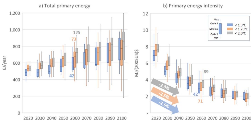
Fig. 4. Global primary energy demand and primary energy intensity of GDP. Arrows on Fig. 4b) show compound average annual reduction in primary energy intensity of GDP over the 2020–2040 period, expressed as a median value across each group of scenarios. Numbers on chart areas refer to number of scenarios in each group for which indicator data is available. Whilst total primary energy is available for all models, global GDP is only reported for 71 of 73 models in the below 1.75 °C group and for 89 models in the below 2 °C group (as shown in Figure S2b, Supplementary Material). Hence primary energy intensity of GDP can only be shown for this reduced number of scenarios.
