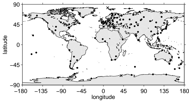
Fig. 1. Ionosonde stations with observations of at least 22 years from the databank of Damboldt and Suessmann (2012a). Dots indicate stations with foF2 and M(3000)F2 data, and crosses indicate stations with foF2 data only.
