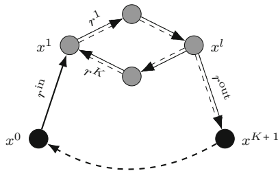
Fig. 4 A disconnected component \mathfrak{d} of damped fluxes, chained in a cycle
