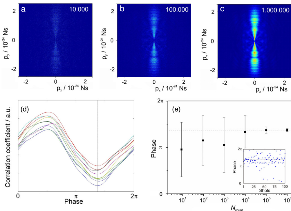
Figure 10. (a)–(c) Single-shot images generated by MC sampling for a given number N_{\text{count}} . (d) Correlation coefficient as defined in the text for a set of seven simulated single-shot images and their comparison to a set of 40 reference images for phases between 0 and 2\pi . The original CEP is indicated by the solid line. (e) Mean value and error in the single-shot CEP determination as a function of N_{\text{count}} for a set of 100 single-shot images. The inset shows an example of the single-shot sampling of the phase for N_{\text{count}} = 10\,000 . The dotted line indicates the original CEP.
