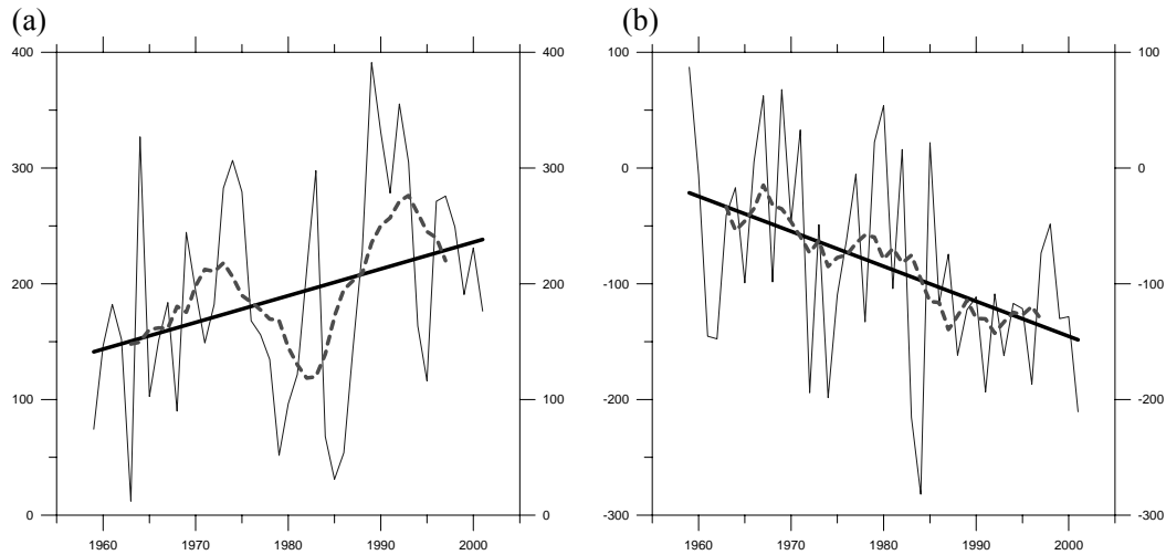
Fig. 9. Same as Fig. 8 over Central Europe (50° N, 10° E) (a) and Labrador (b) at for January.
