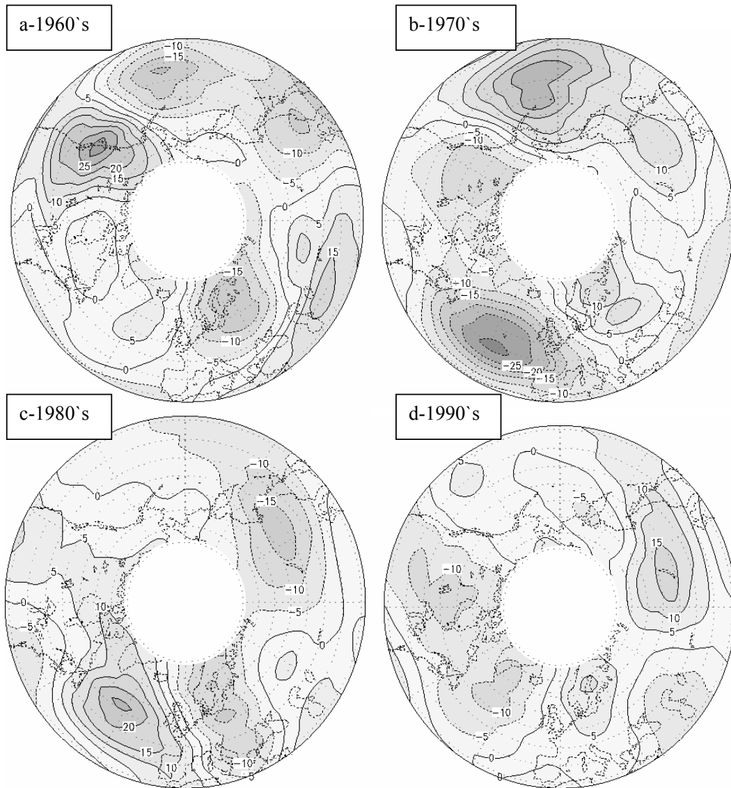
Fig. 5. Model results of mean decadal change in total ozone (DU) for the 1960s (a), 1970s (b), 1980s (c) and 1990s (d) calculated with differences of 5-year averages (end minus beginning of the decade) of geopotential heights for January.
