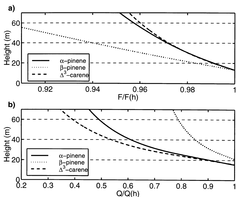
Fig. 7. Vertical profiles of (a) fluxes of \alpha -pinene, \Delta^3 -carene and \beta -pinene, and (b) chemical sink term for the given monoterpenes above the forest at midday, 11 August 1998.
