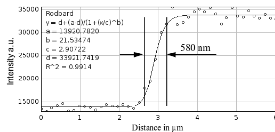
Figure 6. Line plot through the edge of a mesh bar, (black box in figure 5).
