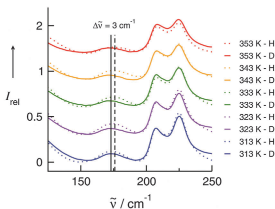
Fig. 2 Far infrared spectra of IL I with protonated (dotted line) and deuterated (full line) hydroxyl groups at cholinium. The resulting redshift of 3\text{ cm}^{-1} could be observed because only the 2-hydroxyethyl group is involved in this vibrational mode and the reduced mass effect becomes significant.
