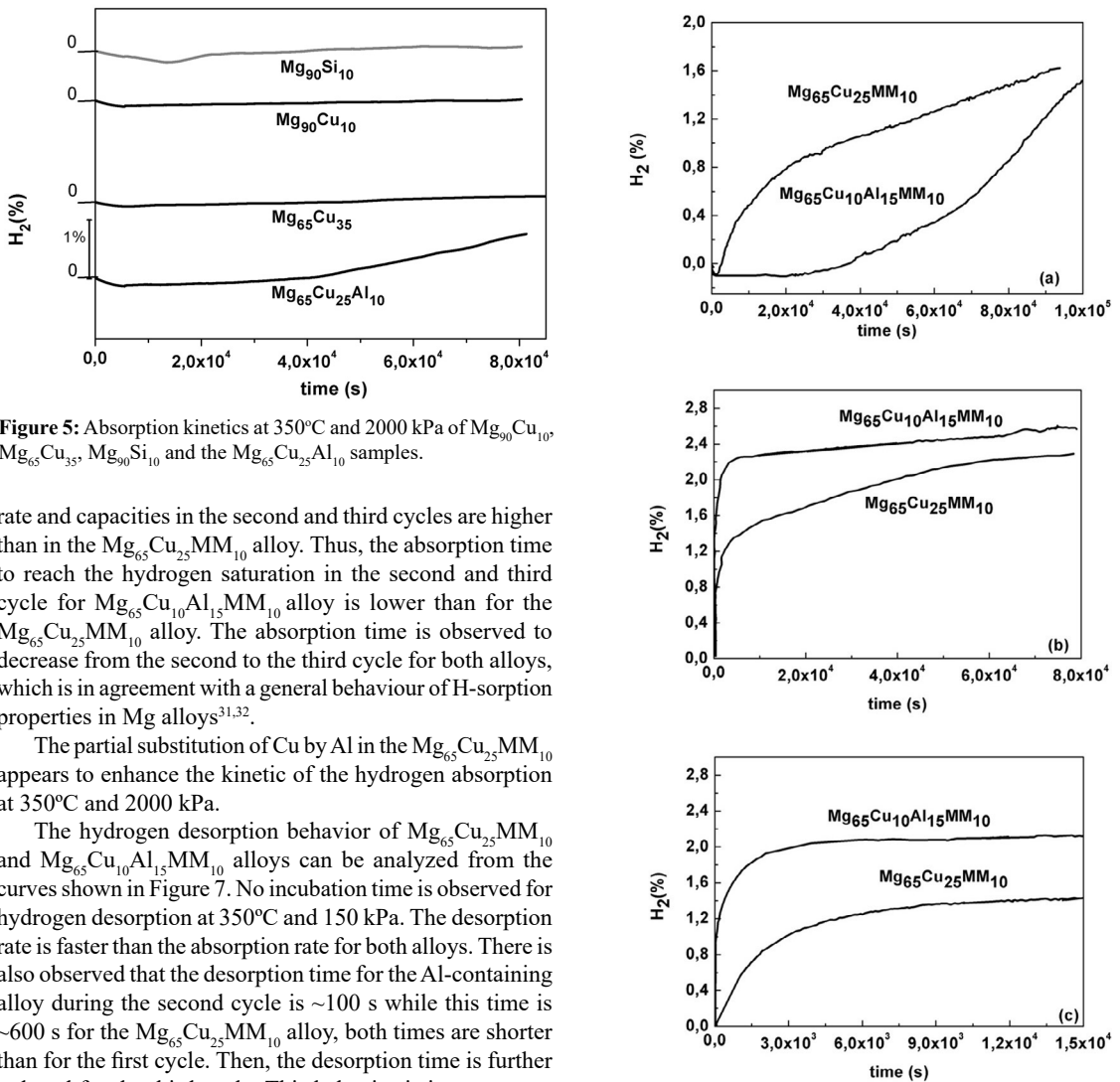
Figure 6: Absorption kinetic at 350 °C and 2000 kPa of the Mg_{65}Cu_{25}MM_{10} and Mg_{65}Cu_{10}Al_{15}MM_{10} alloy; (a) first cycle (activation); (b) second cycle, and (c) third cycle.
