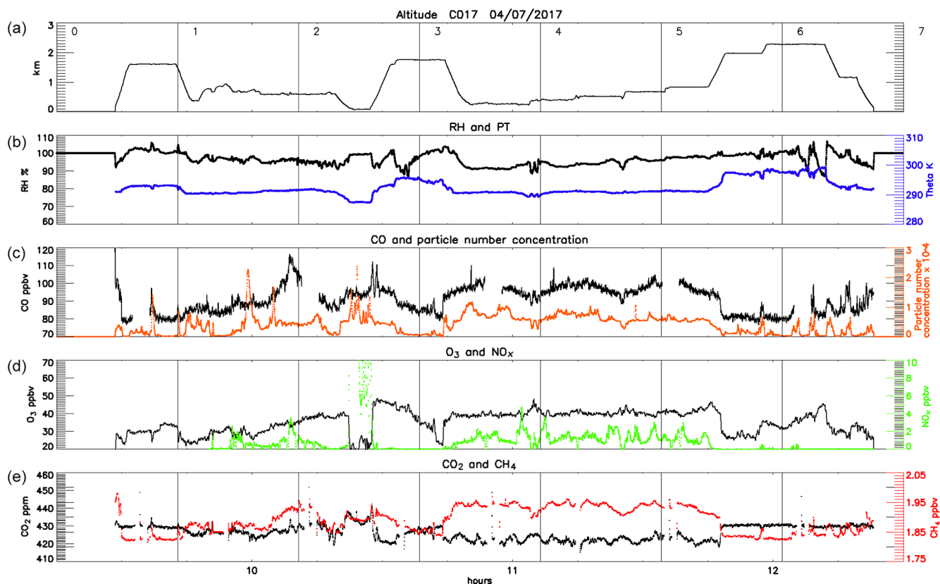
Figure 5. As in Fig. 4 but for the second flight (C017; 4 July, morning).
