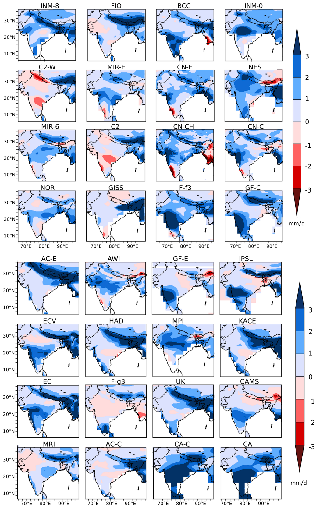
Figure 7. Difference in Indian summer monsoon mean rainfall ( \text{mm d}^{-1} ) for the period 2070–2100 under SSP5-8.5 in comparison to 1985–2015.
