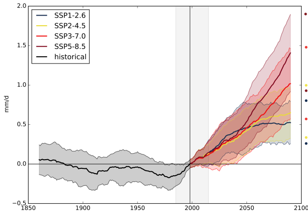
Figure 5. Multi-model mean of Indian summer monsoon rainfall ( \text{mm d}^{-1} ) over the displayed area in Fig. 3 for 1860–2090 relative to the mean (horizontal black line) in 1985–2015 (gray background) for the four scenarios (SSP1-2.6, SSP2-4.5, SSP3-7.0 and SSP5-8.5). The 20-year smoothed time series of one ensemble member per model was used to calculate the multi-model mean. Shading in the time series represents the range of mean plus/minus 1 standard deviation marked with circles on the right side of the figure. Availability of the models is in accordance with Table 1.
