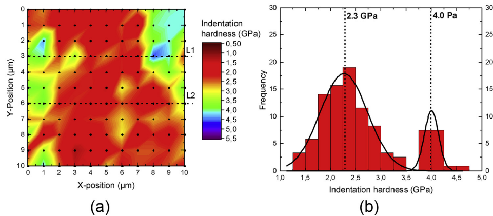
Fig. 1. (a) Indentation hardness map of the Cu-54 at.%Co composite at medium applied strain ( \epsilon = 55 ) as obtained by the grid indentation technique ( 10 \times 10 indents matrix, spacing 1 \mu\text{m} , indentation depth 50 \text{ nm} ) and (b) grid indentation histogram of the dataset illustrating the peaks obtained for the Cu and Co phase and the deconvoluted values of hardness.
