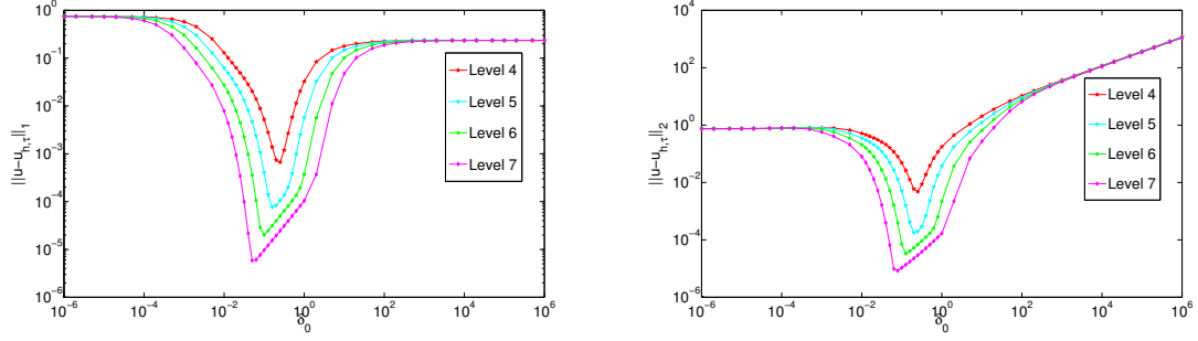
Figure 1: Example 5.2: errors in the norms \|\cdot\|_1 (left) and \|\cdot\|_2 (right) versus the constant \delta_0 for SUPG/cGP(2) on refinement levels 4–7.
