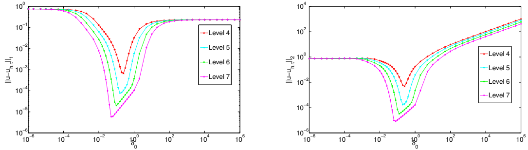
Figure 2: Example 5.2: errors in the norms \|\cdot\|_1 (left) and \|\cdot\|_2 (right) versus the constant \mu_0 for LPS/cGP(2) on refinement levels 4–7.
