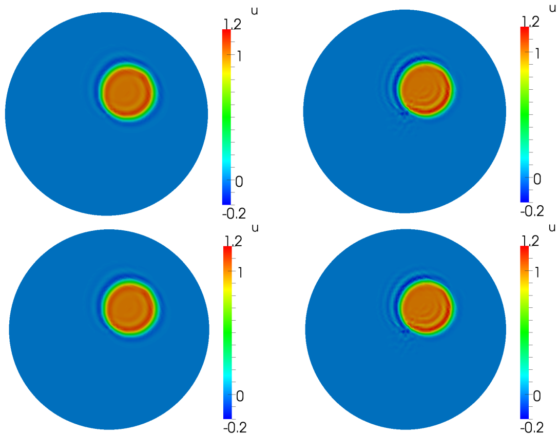
Figure 8: Example 5.3: computed solution with second order elements at t = 20\pi , upper left: SUPG/dG(1), bottom left: SUPG/cGP(2), upper right: LPS/dG(1), bottom right: LPS/cGP(2).
