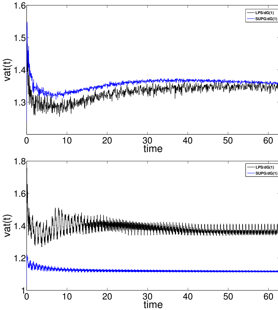
Figure 9: Example 5.3: long time behavior of measure \text{var}(t) for under- and overshoots, computed with second order elements till T = 20\pi , top: problem in unit square with three rotating bodies, bottom: problem in unit circle with one rotating body.
