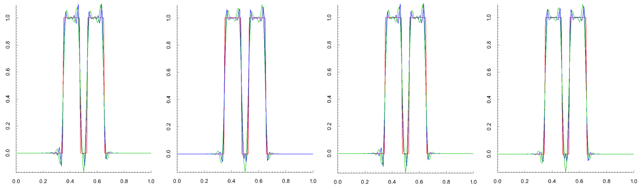
Figure 7: Example 5.3: cut along the line y = 0.75 through the midpoint of the slit cylinder; red: initial condition, blue: solution after one complete revolution ( t = 2\pi ), green: solution after ten complete revolutions ( t = 20\pi ); from left: SUPG/dG(1), LPS/dG(1), SUPG/cGP(2), LPS/cGP(2).
