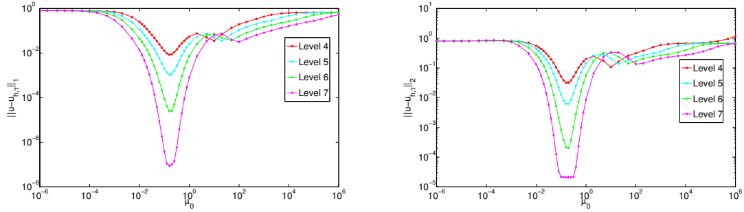
Figure 4: Example 5.2: errors in the norms \|\cdot\|_1 (left) and \|\cdot\|_2 (right) versus the constant \mu_0 for LPS/cGP(2) on refinement levels 4–7.
