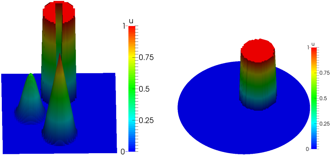
Figure 6: Example 5.3: initial condition; left: problem in unit square with three bodies, right: problem in unit circle with one body.
