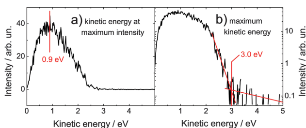
Fig. 5 Time-resolved spectrum of adenosine solution at the temporal overlap ( \pm 0.1 ps) of both pulses (4.66 and 5.21 eV). The maximum kinetic energy is 3.0 eV. The one-color multi-photon signals have been subtracted. Note that the ordinate in (b) is scaled logarithmically.
