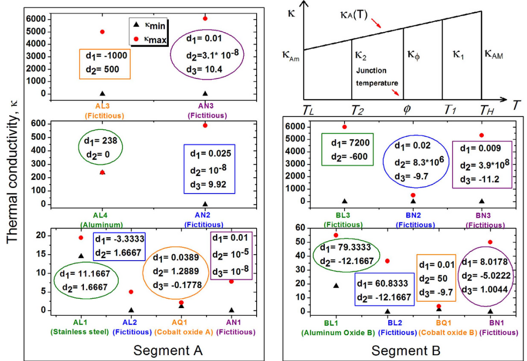
Figure 3. Thermal conductivities of fifteen segment materials. The chemical formula for cobalt oxide A and cobalt oxide B take the form La_{0.7}Sr_{0.3}CoO_3 and LaCoO_3 . For linear segments, \kappa(T) = d_1 + 2d_2T ; for quadratic segments, \kappa(T) = d_1 + d_2T + d_3T^2 ; for nonlinear segments AN1 and BN1, \kappa(T) = d_1 + d_2T^{d_3} ; for nonlinear segments AN2, AN3, BN2, and BN3, \kappa(T) = d_1 + d_2e^{d_3T} . Note that, in all simulations, the grid node for \kappa staggers half grid interval toward right. Hence, for example, for AN3, \kappa(T_H) = 6067.6 = \kappa_{max} , but \kappa_T(1) = 6064.6 , which exhibits a slightly different value. The subscript “M” of \kappa_{AM} shown in the trapezoid stands for “Maximum” (thus “m”=minimum). The variable \kappa_{AM} is shown in the figure merely for the sake of completeness. It is actually not needed in the derivation of Eq. (20).
