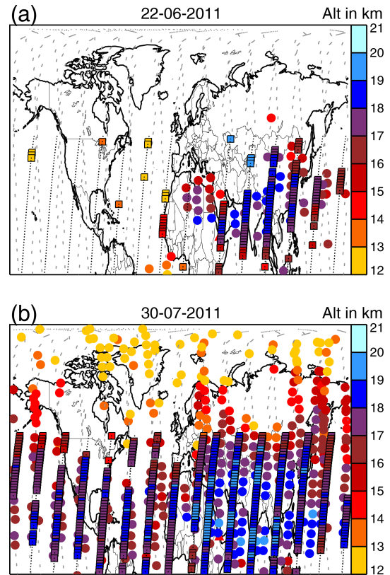
Figure 7. Sulfate aerosol detected by MIPAS (circles) and CALIOP (squares) (a) 10 d and (b) 48 d after the Nabro eruption. The MIPAS orbit tracks, indicated by grey dashes, reach up to 90^\circ N and the CALIOP orbit tracks of available aerosol data are indicated by black dots. The colours indicate the layer top height. For CALIOP aerosol detections an altitude-variable extinction threshold that is 3 \times 10^{-3} \text{ km}^{-1} at 18 km was used.
