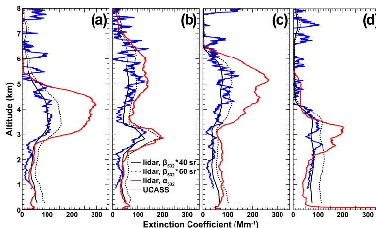
Figure 9. Aerosol extinction coefficient profiles from UCASS (red) and the Raman lidar Polly XT at Limassol. Lidar profiles refer to extinction coefficients obtained using the Raman method (blue) or by multiplying the aerosol backscatter coefficient derived without the use of Raman signals with lidar ratios of 40 sr (solid black line) and 60 sr (dotted black line). Panels refer to the first (a), second (b), third (c), and fourth (d) UCASS launches (see Fig. 1 and Table 1).
