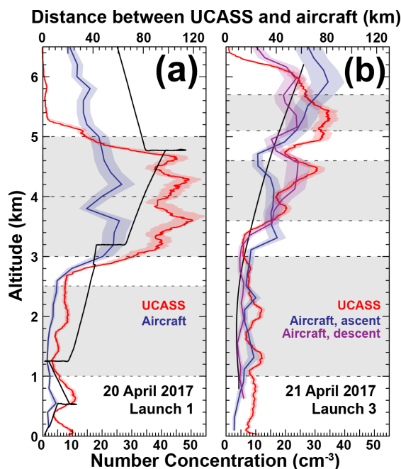
Figure 5. Total number of particles in the diameter range from 0.6 to 13.9 \mu\text{m} counted by UCASS (red) and with the CAPS (CAS) instrument aboard the Falcon aircraft (blue and purple, size range from 0.79 to 14.0 \mu\text{m} ; shading marks the standard deviation obtained as median minus 25th percentile and 75th percentile minus median) measured (a) during the first UCASS launch on 20 April 2017 and (b) during the third UCASS launch on 21 April 2017. Red shaded areas refer to the effect of a counting uncertainty of 8 % ( y error) as stated in Smith et al. (2019). The black lines mark the horizontal distance between the location of the observations from the UCASS and aircraft. Grey areas refer to the height layers considered in Fig. 6.
