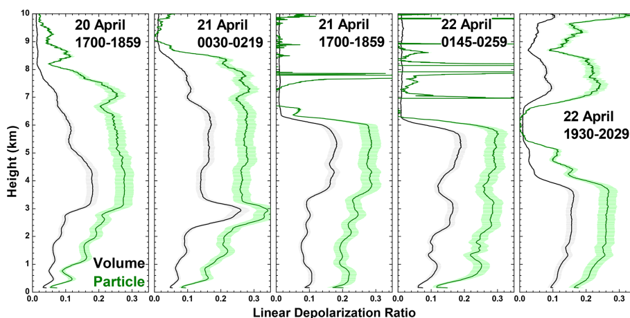
Figure 2. Profiles of the linear volume depolarization ratio (black line with grey error range) and the particle linear depolarization ratio (dark green line with light green error range) measured by the Polly XT lidar around the times (see Table 1) of the UCASS launches marked in Fig. 1.
