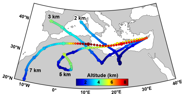
Figure 4. The 120 h HYSPLIT backward trajectories starting over Limassol at 01:00 UTC on 21 April 2017. Colour coding refers to the height of the trajectories. Intervals of 12 h are marked by increased circle size. The numbers in the plot refer to the arrival height over Limassol.
