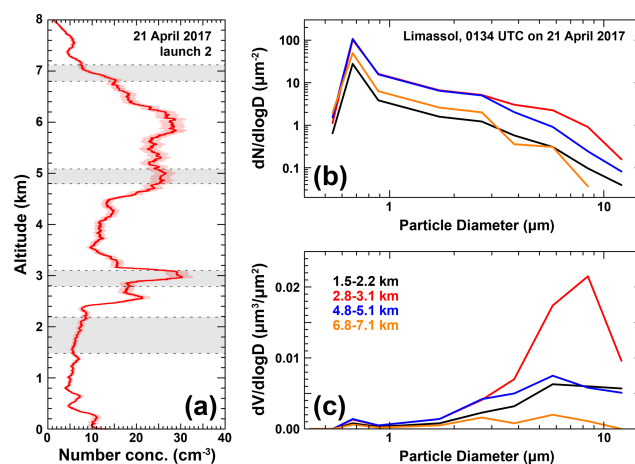
Figure 8. UCASS measurements during the second launch at 01:34 UTC on 21 April 2017 from Limassol: (a) height profile of the total particle number concentration as in Fig. 4 and (b) particle number and (c) volume–size distributions averaged over four selected height levels as indicated in (a).
