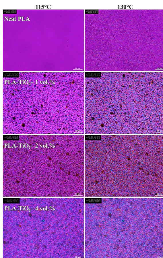
Figure 1: The optical micrographs of the spherulites of PLA with different TiO_2 loadings obtained from non-isothermal cold crystallization during the second heating process at 115°C and 130°C (Scale bar, 50 \mu m ).
