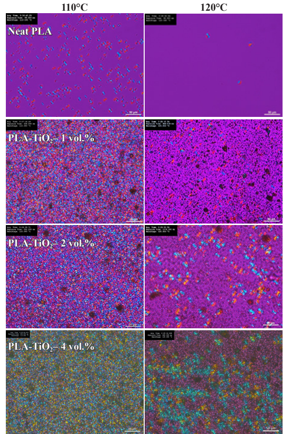
Figure 3: The optical micrographs of the spherulites of PLA with different TiO 2 loadings obtained from isothermal crystallization at temperature 110°C and 120°C with crystallization time 10 minutes (Scale bar, 50 µm).
