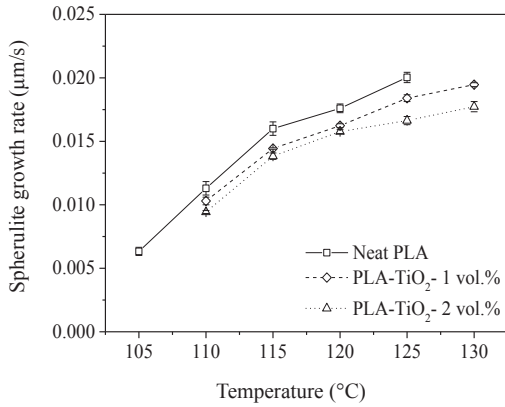
Figure 2: The spherulite growth rate of neat PLA and its nanocomposites with different TiO 2 nanoparticles loading at various crystallization temperatures.
