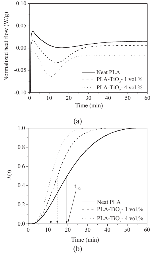
Figure 5: Typical crystallization exothermic curve (a) and relative crystallinity, X(t) as a function of crystallization time (b) of PLA with different TiO 2 loadings, T i = 110°C.
