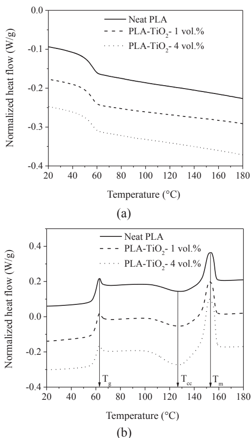
Figure 4: DSC thermograms of PLA with different TiO 2 loadings obtained from first cooling run (a) and second heating run (b).
